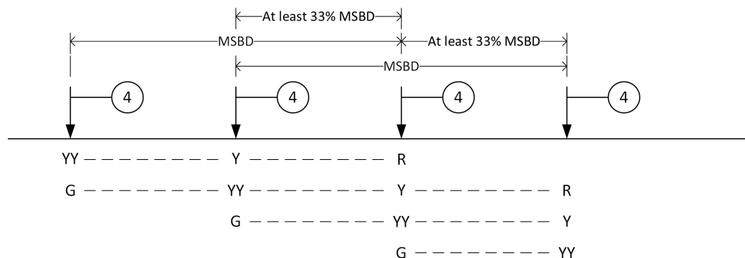
Figure 8: An example of a 4-aspect sequence
