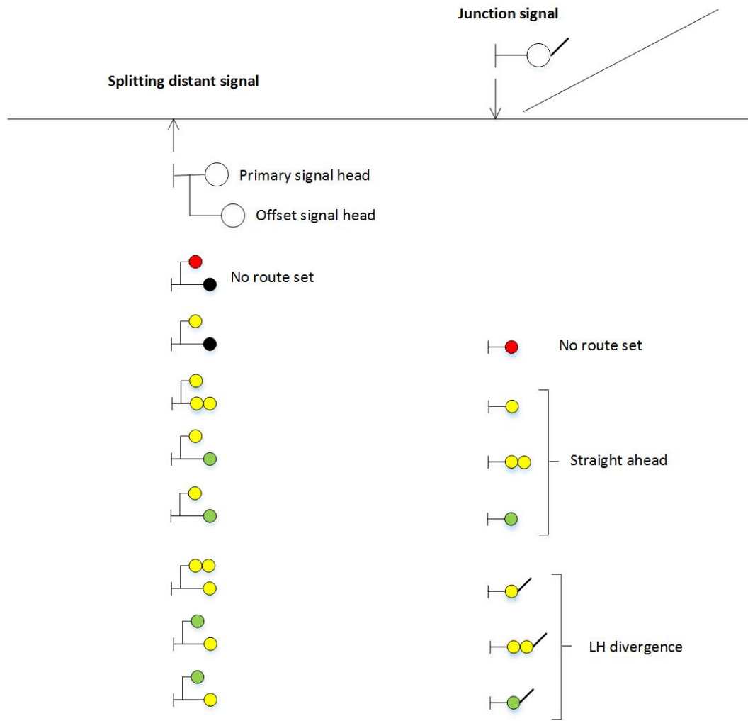
Figure 17: Splitting distant signal positioned on the right-hand side of the line with a left-hand diverging junction
