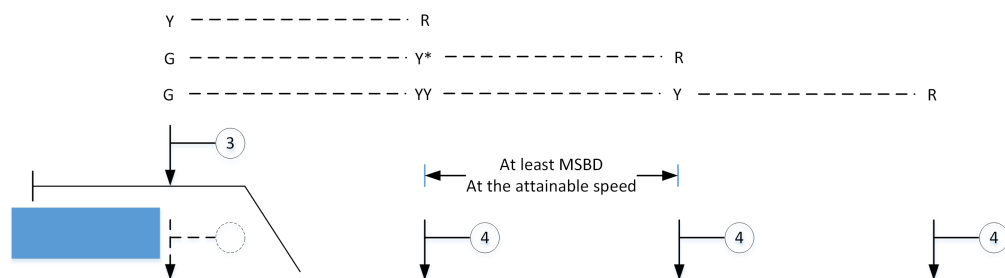
Figure 9: An example showing a 4-aspect sequence that omits the YY aspect for trains starting from a bay platform
