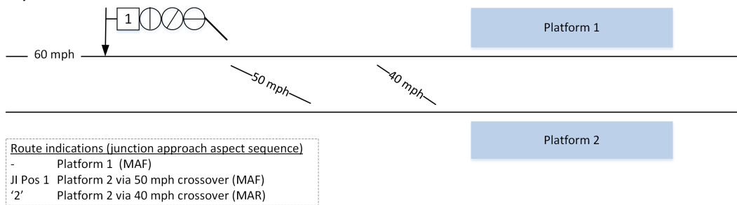
Figure 10: Example of indicating alternative paths using different types of route indications
