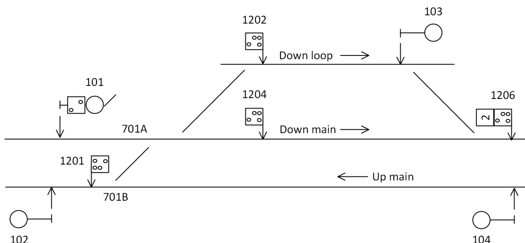
Figure 2: Example of a preceding shunt signal
