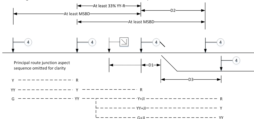
Figure 15: A typical MAY-YY aspect sequence
