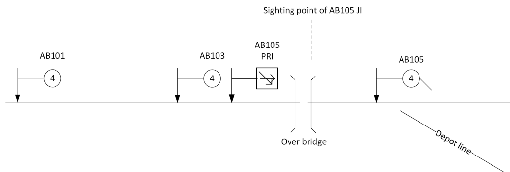
Figure 12: Example of a PRI on the approach to a junction signal
