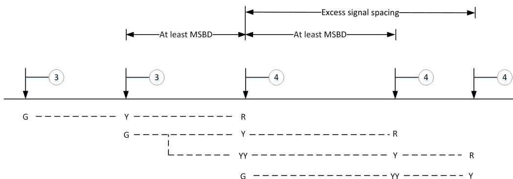
Figure 4: Example of a 3-aspect to 4-aspect transition with excess signal spacing
