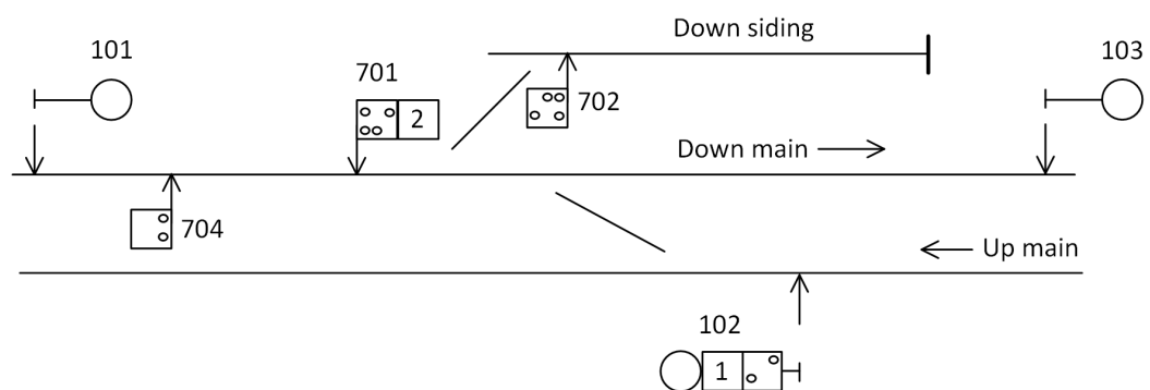
Figure 1: Example of a preset shunt signal
