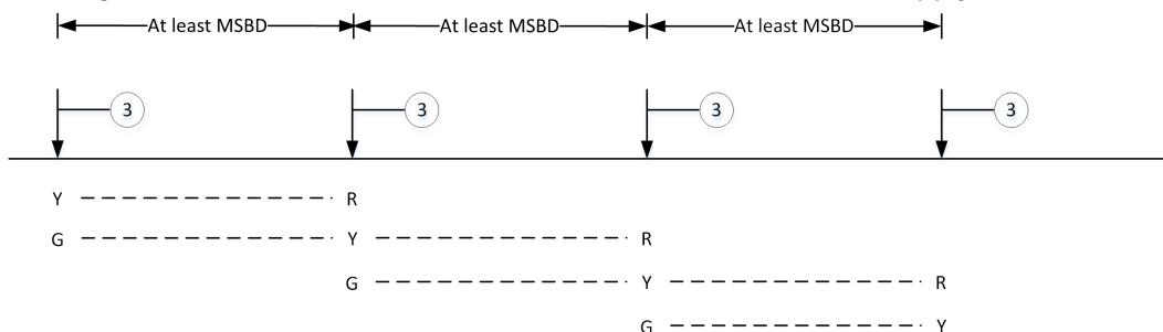
Figure 7: An example of a 3-aspect sequence presented by colour light signals
