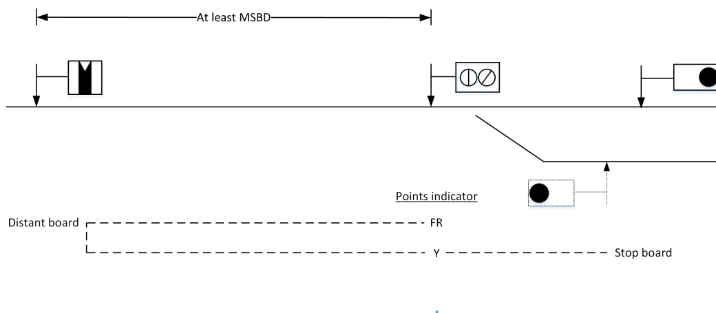
Figure 20: A typical sequence of indications at locally monitored facing points
