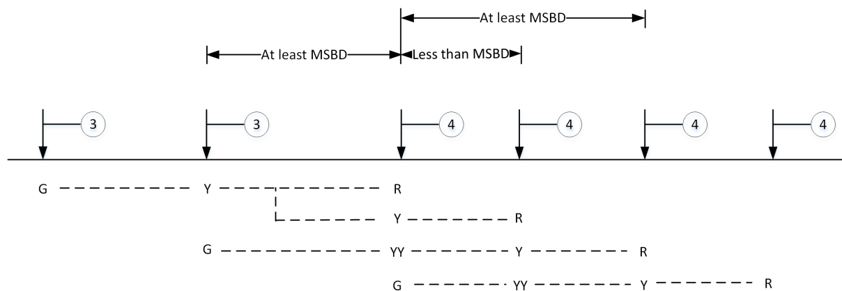
Figure 5: Example of applying an approach release from red control at a 3-aspect to 4-aspect transition
