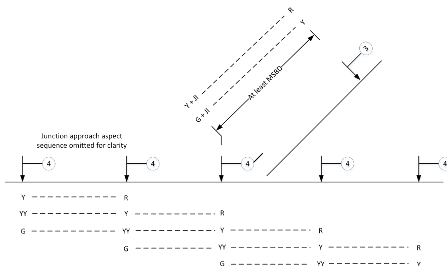
Figure 6: A 4-aspect to 3-aspect signalling transition at a diverging junction
