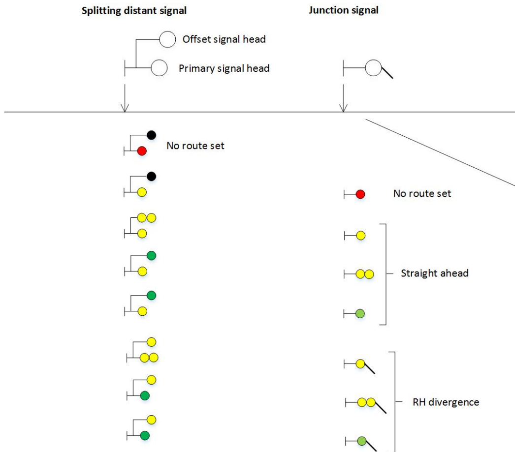
Figure 18: Splitting distant signal positioned on the left-hand side of the line with a right-hand diverging junction
