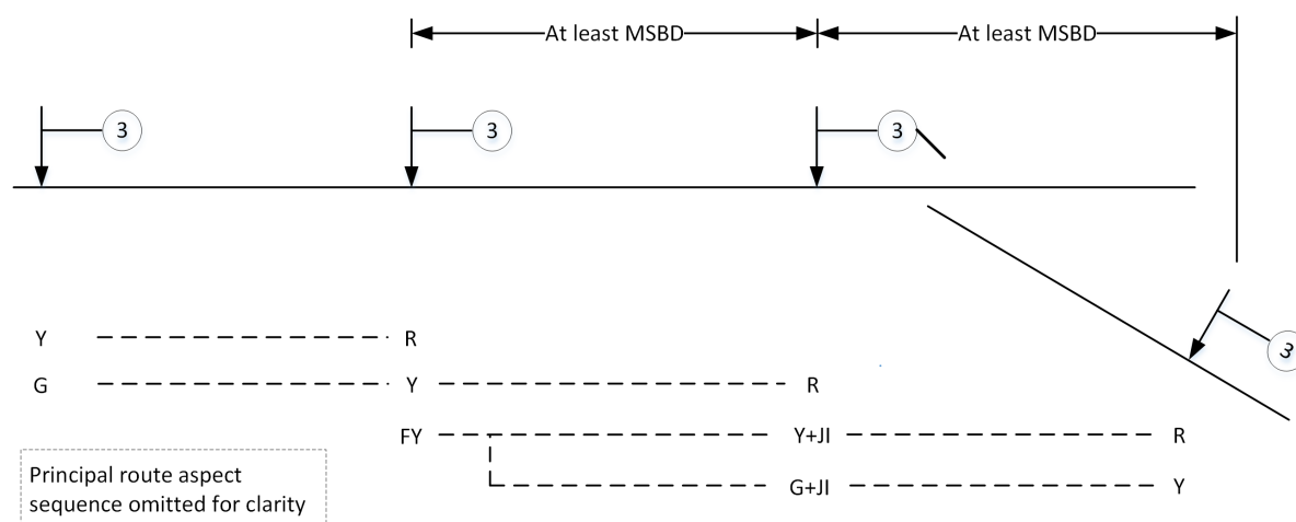
Figure 13: A typical MAY-FA3 aspect sequence for a right hand diverging junction
