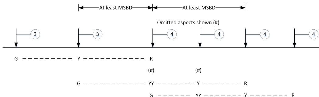
Figure 3: Example of a 3-aspect to 4-aspect transition omitting a main stop aspect
