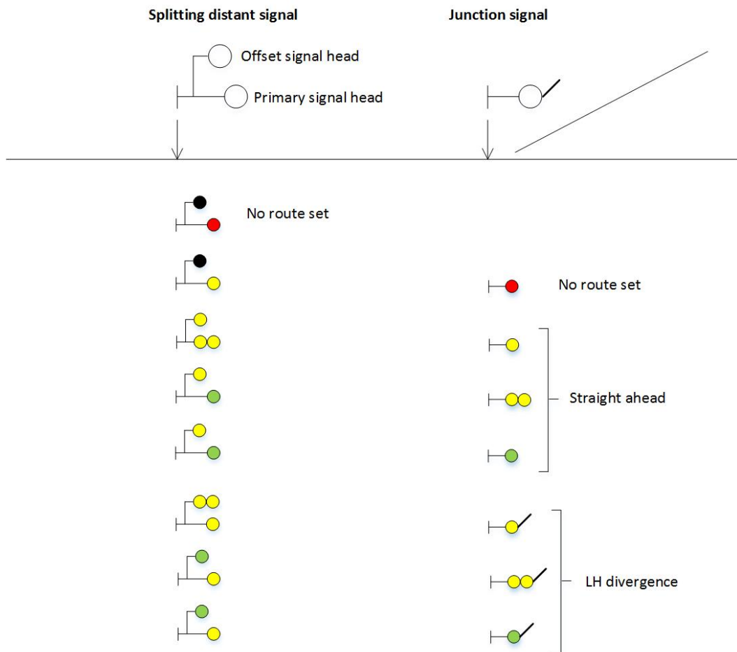
Figure 16: Splitting distant signal positioned on the left-hand side of the line with a left-hand diverging junction
