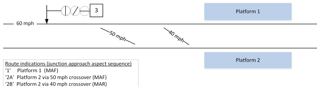
Figure 11: Example of indicating alternative paths using alphanumeric route indications
